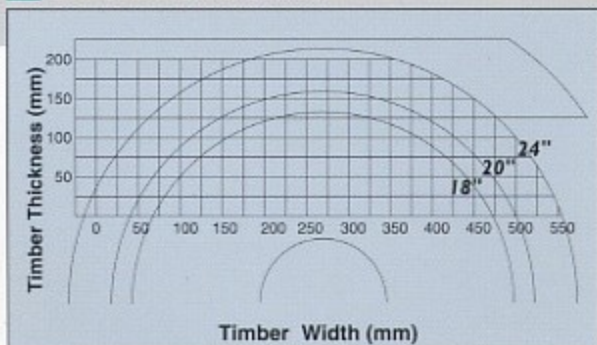
24" CAPACITY CHART
